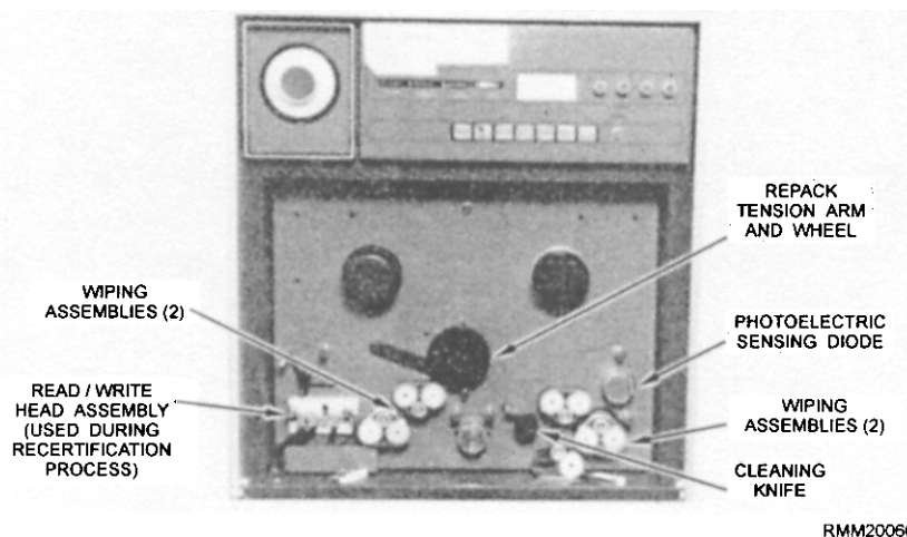
Figure 2-12.—Tape cleaner/certifier.
