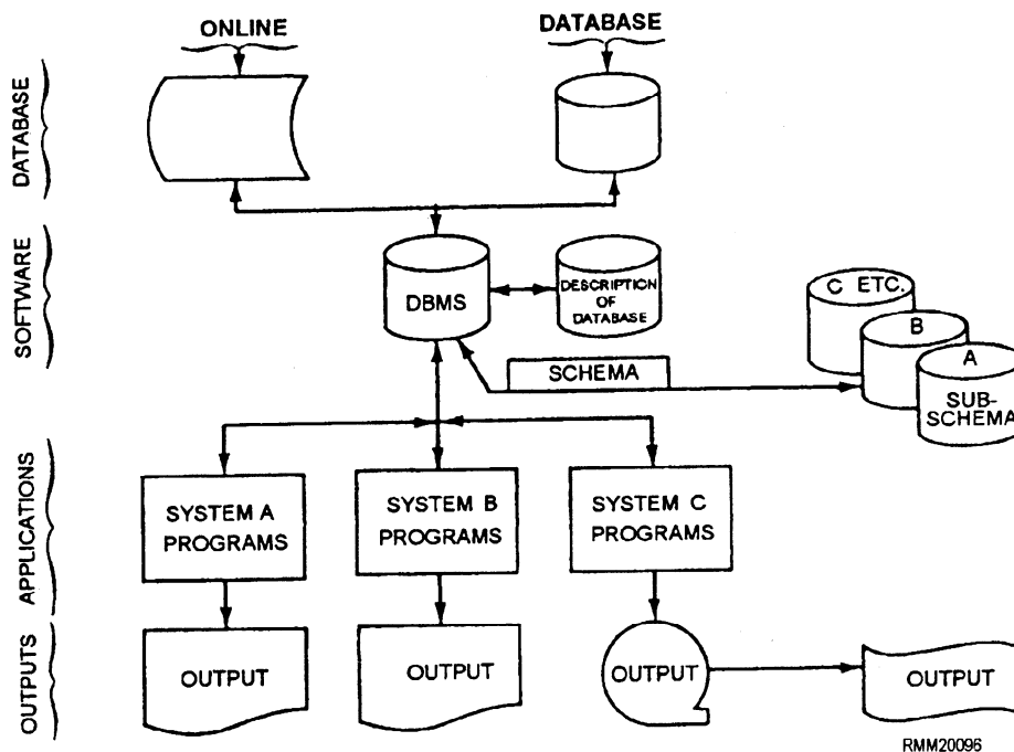
Figure 3-14.—A database management system (DBMS).
