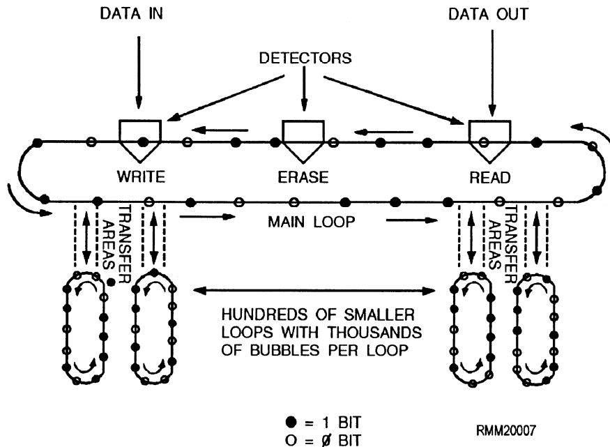
Figure 1-6.—Bubble memory.
